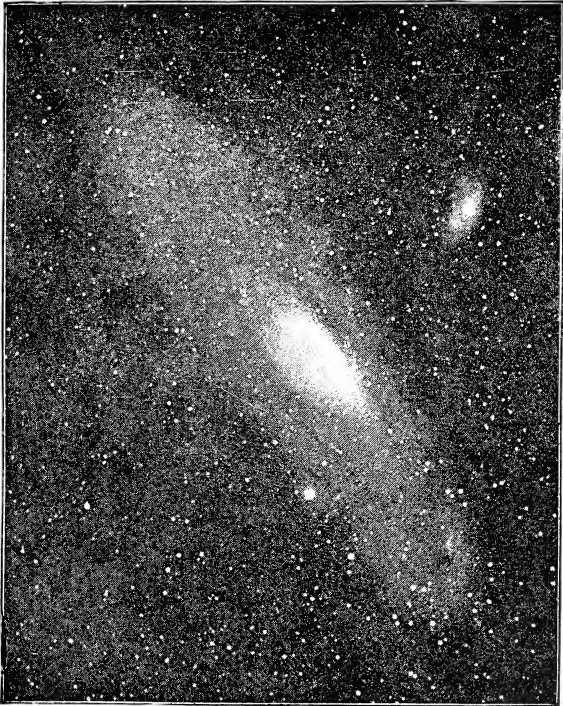
Fig. 88.—Taken from Mr. Roberts's Photograph of the Great Nebula in Andromeda.
